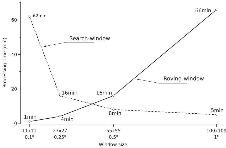
Fig. 4. Processing time for mean slope operation, using roving-windows and search-windows, according to window size.
