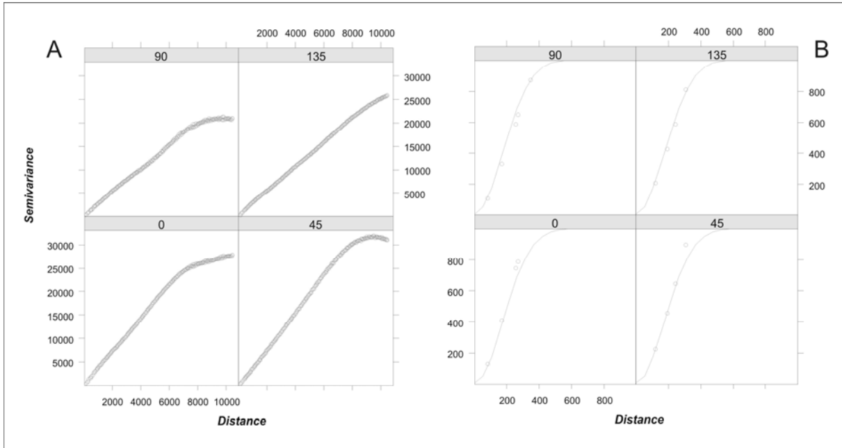
Fig.2: Exploratory analysis of Japi area. a) complete variograms; b) initial portion of the variograms (Gaussian model, sill=950, range=245).
