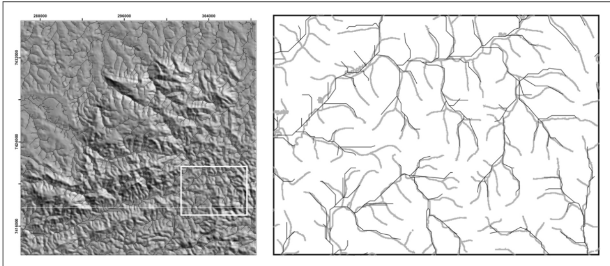
Fig.5: DEM-derived drainages (black lines) overlaid on drainages of 1:50,000 topographic map (grey lines).
