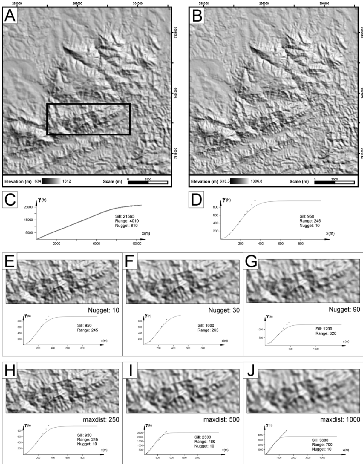
Fig.3: Results of analysis for the Japi area. a) original SRTM 3arcsec data; b) resampled 1arcsec data; c) full variogram; d) short-distance variogram; e) kriged surface with nugget= 10m^2 ; f) kriged surface with nugget= 30m^2 ; g) kriged surface with nugget= 90m^2 ; h) kriged surface with maxdist=250m ; i) kriged surface with maxdist=500m ; j) kriged surface with maxdist=1000m .
