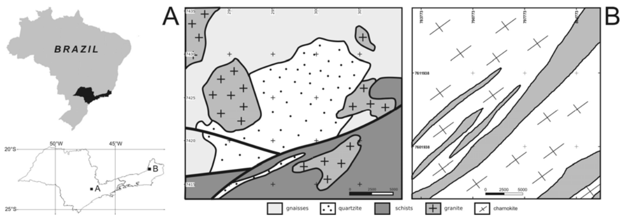
Fig.1: Location and simplified geology of study areas. A) Japi area. B) Mantiqueira area.
