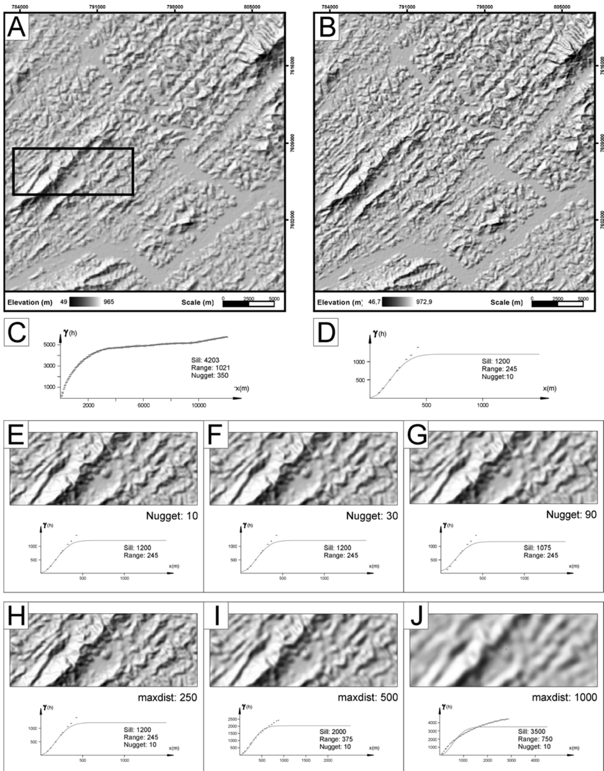
Fig.4: Results of analysis for the Mantiqueira area. a) original SRTM 3arcsec data; b) resampled 1arcsec data; c) full variogram; d) short-distance variogram; e) kriged surface with nugget= 10\text{m}^2 ; f) kriged surface with nugget= 30\text{m}^2 ; g) kriged surface with nugget= 90\text{m}^2 ; h) kriged surface with \text{maxdist}=250\text{m} ; i) kriged surface with \text{maxdist}=500\text{m} ; j) kriged surface with \text{maxdist}=1000\text{m} .
